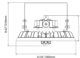
Surface Mount
