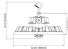
Eye Hook
